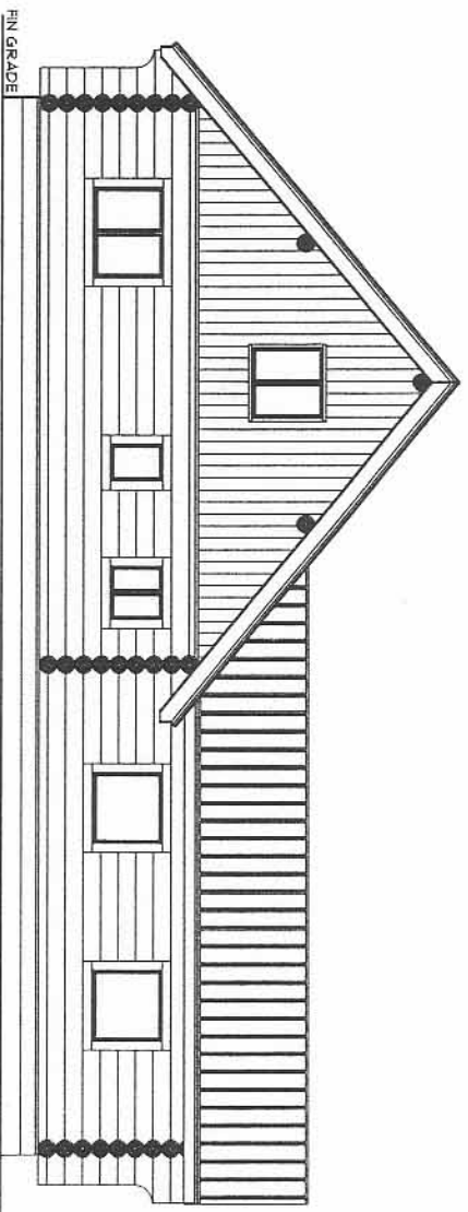
REAR ELEVATION
